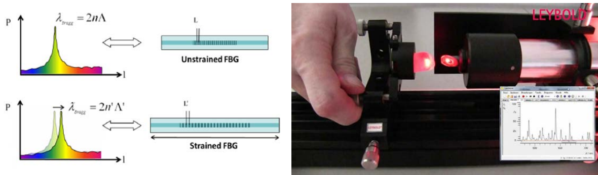
Fig. 2. Experiments with an open HeNe laser and a fiber Bragg grating
